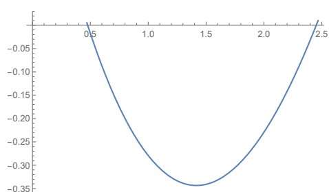
Fig. 1. (L_1 - k) \cos \sqrt{k} + L_2(x) \sqrt{k} \sin \sqrt{k}
