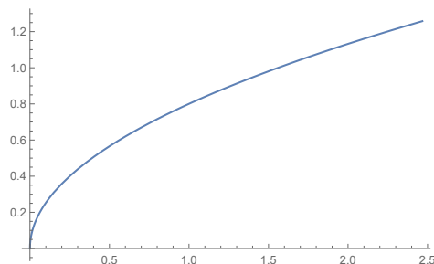
Fig. 2. \sqrt{k} - \lambda_1 \sin \sqrt{k} \xi
